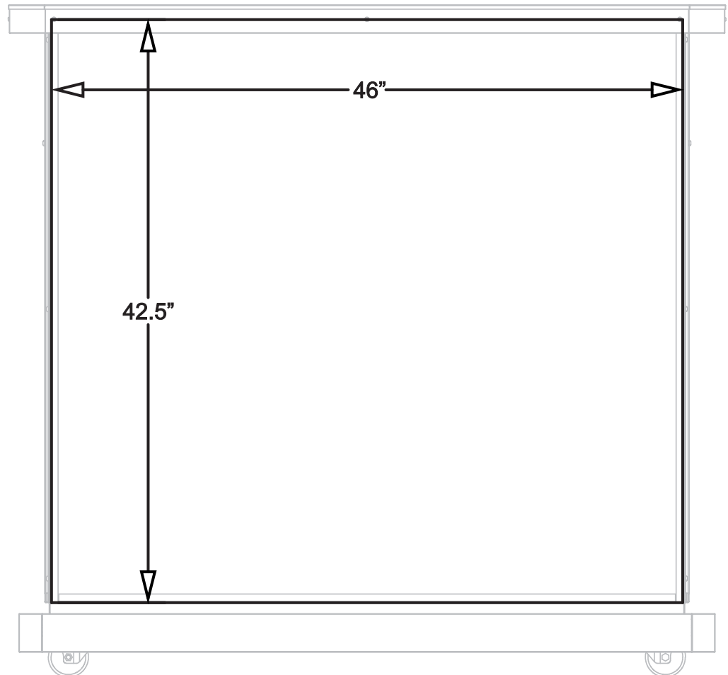
Back Acrylic Panels Dimensions
